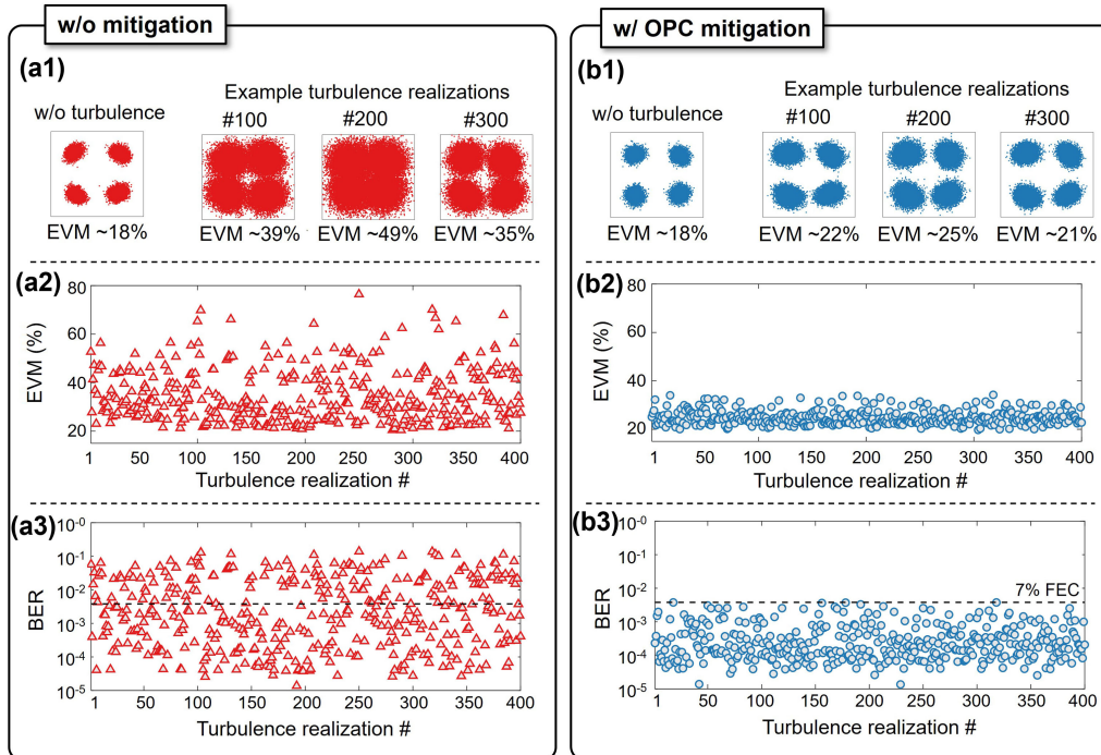
Fig. 6. Experimental results for 8-Gbit/s QPSK data transmission in a coherent FSO link under dynamic turbulence without mitigation and with OPC mitigation. Results are measured for 400 different turbulence realizations when the turbulence phase screen rotates at 2 round/sec., including data constellations in (a1) and (b1), EVM performance in (a2) and (b2), and BER performance in (a3) and (b3). Note that we measure the results with and without mitigation at separate times due to the limitations of our measurement setup. Therefore, the results with the same realization label may correspond to different turbulence realizations and are difficult to be directly compared.
