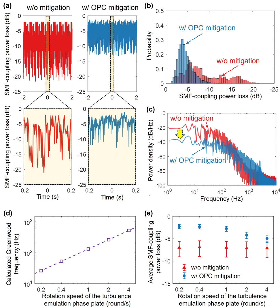
Fig. 5. Experimental results of SMF-coupling power loss of the received data beam under dynamic turbulence. (a) Power fluctuation, (b) probability distribution, and (c) density spectrum of the SMF-coupling loss without and with phase conjugation mitigation. The results in (a–c) are for the turbulence phase screen ( r_0 = 0.6 mm) rotating at 2 round/sec. The power loss is measured by a fiber-coupled photodiode with a 10 kHz bandwidth at a sampling rate of 900 k sample/sec. (d) Calculated Greenwood frequency for different rotation speeds of the turbulence phase screen. (e) Average SMF-coupling loss for different rotation speeds of the turbulence phase screen. The error bars show the standard deviation of the measurements.
