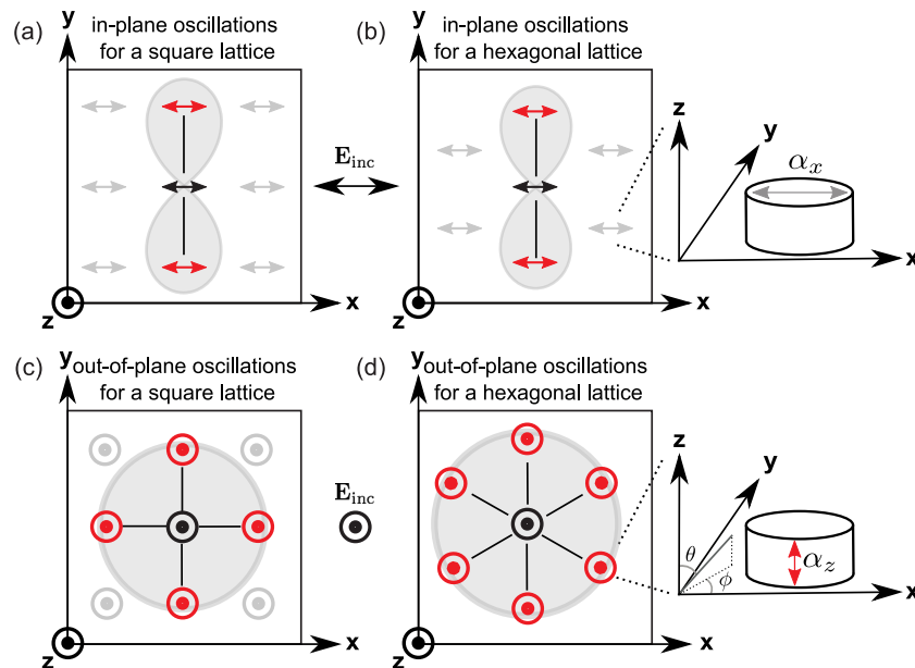
Fig. 1. Schematic diagram showing the dominant nearest neighbors for in-plane [(a) and (b)] and out-of-plane [(c) and (d)] dipole oscillations in square [(a) and (c)] and hexagonal [(b) and (d)] lattices. The light grey shaded region in each panel shows the scattering pattern of the nanoparticle at the center of the array [shown as a black arrow in (a) and (b) and a black circled dot in (c) and (d)]. Red arrows [(a) and (b)] and red circled dots [(c) and (d)] indicate the most strongly coupled nearest neighbors, and solid lines show the directions in which inter-particle coupling is strongest. Grey arrows [(a) and (b)] and grey circled dots [(c) and (d)] show neighbors for which the coupling is weak. For in-plane oscillations [(a) and (b)], strong coupling occurs only in one specific direction (indicated by solid lines), whereas for out-of-plane oscillations [(c) and (d)], strong coupling occurs in all directions within the plane of the array (as shown by solid lines). The insets schematically show the relevant polarizability components for in-plane ( \alpha_x ) and out-of-plane ( \alpha_z ) oscillations.
