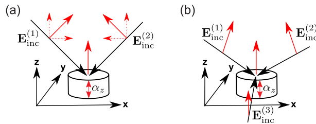
Fig. 4. More efficient coupling schemes for (a) square and (b) hexagonal arrays with out-of-plane oscillations. (a) If the incident fields are out-of-phase, the in-plane (out-of-plane) field component of the incident waves interfere destructively (constructively), thus making the coupling into out-of-plane oscillations dominant. (b) Similar to square lattices, hexagonal lattices can be efficiently excited using three incident fields.
