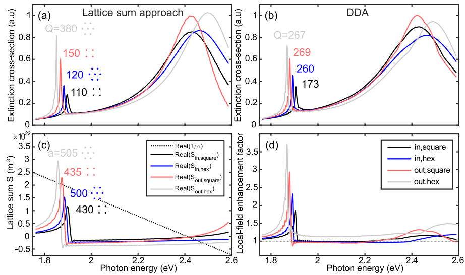
Fig. 3. The extinction spectra for the array periods of a = 430 nm, 500 nm, 435 nm, and 505 nm, calculated using the lattice sum approach (a) and DDA (b). The slightly different periods were chosen to separate the peaks on the graph for better clarity. The calculated Q-factors of the SLRs are shown next to their corresponding peaks in (a) and (b). These results can be understood in terms of the lattice sums, shown in (c). Strong SLRs occur when the real part of the lattice sum S_i and 1/\alpha (shown with the dotted line) cross. Therefore, larger lattice sums can give rise to stronger SLRs. The enhancement of the mesoscopic local field acting on an individual nanoparticle by the array and its resonances is shown in (d).
