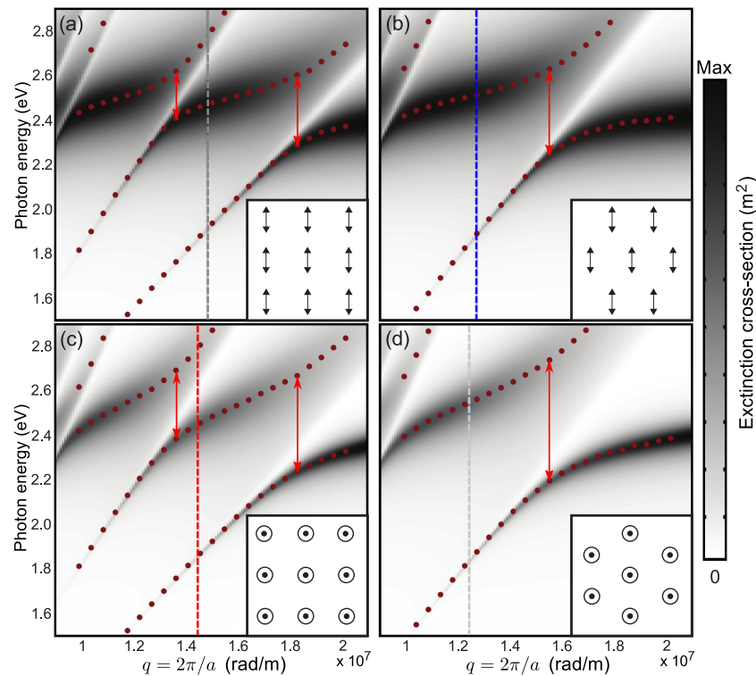
Fig. 2. Extinction cross-section as a function of the incident photon energy and the inverse array periodicity q = 2\pi/a , plotted for (a) in-plane square, (b) in-plane hexagonal, (c) out-of-plane square, and (d) out-of-plane hexagonal arrays. Dark-red filled circles follow the local maxima of the extinction and display the dispersion relation of the resonances. For the out-of-plane resonances, the stronger inter-particle coupling results in larger avoided crossings between the modes, visualized by red arrows. The special cases treated in Fig. 3 are indicated by colored dashed lines.
