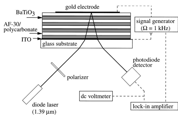
FIG. 2. Sample geometry and experimental arrangement used to measure the electro-optic response. The variation of the reflectivity of the structure is measured as a function of the applied voltage.
