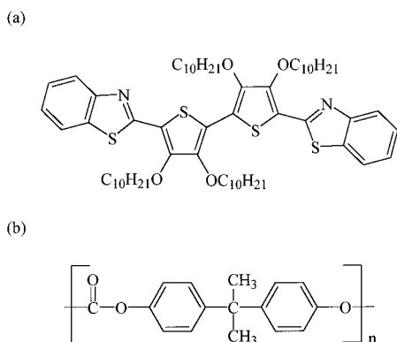
FIG. 3. Chemical structure (a) of the electro-optically active dopant molecule 5-benzothiazol-2-yl-2-[5-benzothiazol-2-yl-3,4-didecyloxy (2-thienyl)]-3,4-didecyloxythiophene, and (b) of the polycarbonate host.
