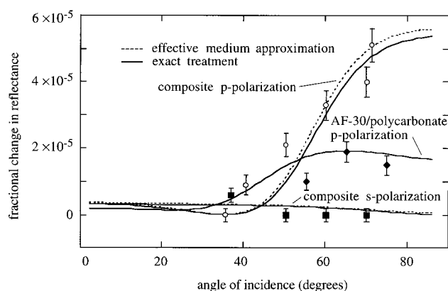
FIG. 4. Fractional change in reflectance plotted as a function of the angle of incidence both for a layered composite material and for a homogeneous layer of the doped polycarbonate material. The continuous curves represent theoretical predictions calculated both using the effective medium approximation and taking explicit account of the layered nature of the material sample. Each theoretical curve depends on one free parameter, the value of \chi^{(3)} . The values of \chi^{(3)} determined from these fits are quoted.
