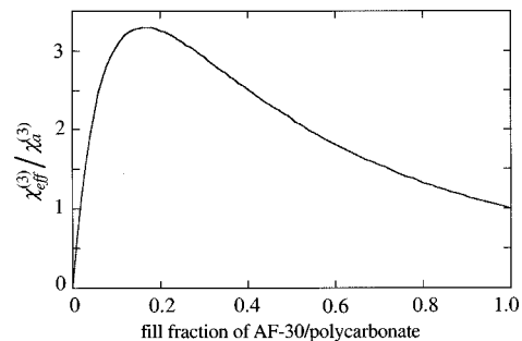
FIG. 1. Predicted enhancement of the electro-optic response plotted as a function of the fill fraction of the doped-polycarbonate constituent of the layered composite material.
