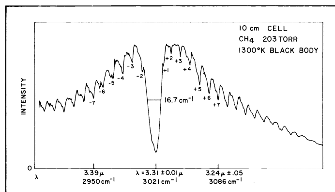
Figure 5. The absorption spectrum of methane measured with the upconverter of Abbas, et al, 28 showing the P, Q, and R branches. The upconverter spectral resolution was \sim 2.7 \text{ cm}^{-1} . 40 minutes of integration were required to take this spectrum.
