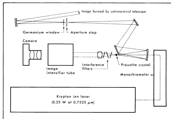
Figure 6. 10 \mu\text{m} imaging upconverter of Boyd. 29 The monochromator is used to eliminate background light from the laser discharge tube. Collimated infrared radiation is mixed with the laser beam in the proustite crystal. The interference filters pass the sum frequency while rejecting the laser frequency, providing a factor of 10^{18} discrimination between the two frequencies. The sum frequency image is amplified by the image intensifier tube and recorded photographically.
