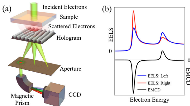
Figure 10. Probing materials with twisted electrons. (a) Illustration of an EMCD (Electron Magnetic Circular Dichroism) apparatus. A sample is exposed to an electron beam which results in the scattering of the incident electrons. A phase-flattening scheme consisting of a hologram and an aperture is then used to post-select electrons with a certain OAM value imparted by the material. A magnetic prism and a CCD camera are then used to acquire the electron energy spectrum of a particular OAM component. (b) Sketch of typical data for the electron energy loss spectra (EELS) and the corresponding EMCD spectrum in an EMCD experiment. The EELS depict the energy spectra of scattered electrons with opposite OAM values and thereby of opposite handedness (left and right). The EMCD spectrum, which corresponds to the difference between the two EELS spectra, exhibits the asymmetry between the scattered OAM components and thereby the material's magnetic properties.
