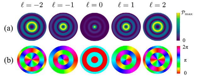
Figure 1. Transverse profile of Bessel electron waves. (a) Transverse probability density function of Bessel beams \psi_{\ell, k_\rho}^{\text{Bessel}} and (b) their corresponding transverse phase profiles plotted in hue colours.
