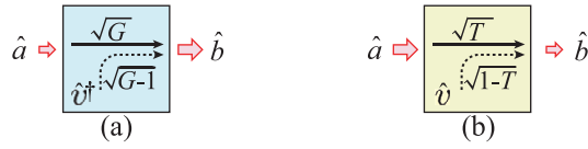
Figure 1. Quantum model of an ideal linear amplifier (a) and an attenuator (b). Here and in figure 2, we use the symbol \hat{v} to designate an internal noise source \hat{c} that is in the vacuum state.
